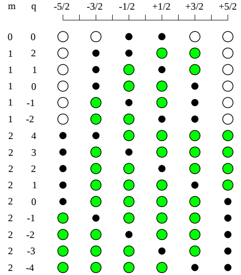
FIG. 4: Psinon vacuum ( m = 0 ) for N = 8 , M_z = 2 and complete set of 2m -psinon excitations with m = 1, 2 and wave numbers q \equiv k - k_G (in units of 2\pi/N ). The positions of the magnons (small circles) are determined by the I_i 's and the positions of the spinons (large circles) by the I_i vacancies. A subset of the spinons are the psinons (green circles).
