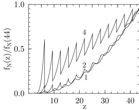
Figure 3. Normalized functions f_N(z) for \sigma(p_F) , (18), f_N(z)/f_N(z=44) , at y = R/L = 1 . Curves 1 and 2 (correlators (1), (2) with \mu = \frac{1}{2} ; f_N(44) = 5 \cdot 10^3 ; 2.5 \cdot 10^2 ) exhibit suppressed usual QSE peaks at small z that gradually transform at higher z into the new QSE oscillations with larger period. Curve 4 for surfaces with power spectrum (4) ( \lambda = 0 ; f_N(44) = 20.2 ) exhibits usual QSE.
