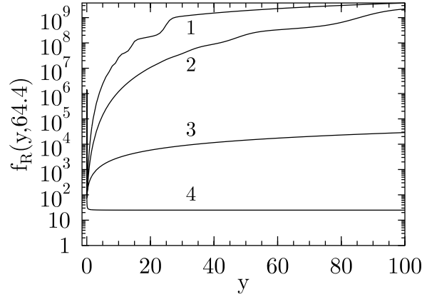
Figure 2. Functions f_R(y) for \sigma(R) , (17), at z = 64.4 . Curves 1 and 2 (correlators (1) and (2) with \mu = \frac{1}{2} ) exhibit new QSE (steps). Curves 3,4 (correlators (4), \lambda = \frac{1}{2}; 0 ) are smooth in accordance with usual QSE.
