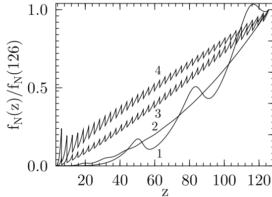
Figure 4. f_N(z)/f_N(z=126) for y = R/L = 20 . Curves 1,2 (correlators (1) and (2), \mu = \frac{1}{2} ; f_N(126) = 1.1 \cdot 10^9 ; 4.5 \cdot 10^7 ) exhibit well-developed new QSE oscillations. Curves 3,4 for correlators (4) with \lambda = \frac{1}{2} ; 0 ( f_N(126) = 1.4 \cdot 10^4 ; 47) still exhibit usual saw-like QSE.
