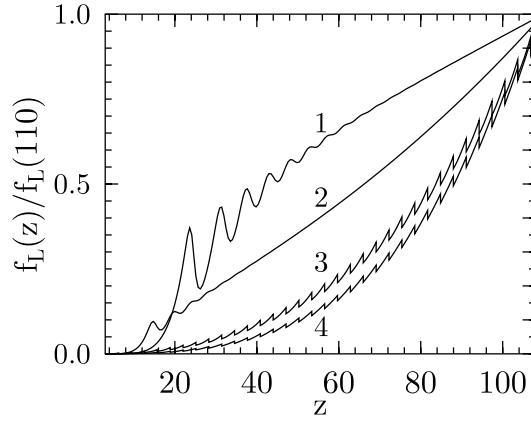
Figure 1. Normalized functions f_L(z) for \sigma(L) , (10), f_L(z)/f_L(z=110) , at x=200 . Curves 1 and 2 (correlators (1) and (2) with \mu = \frac{1}{2} ; f_L(110) = 6.9 \cdot 10^4 ; 7.5 \cdot 10^3 ) exhibit new type of QSE oscillations. Curves 3,4 for surfaces with power spectrum (4) ( \lambda = \frac{1}{2} ; 0; f_L(110) = 3.9 \cdot 10^2 ; 1.3 \cdot 10^1 ) exhibit usual saw-like QSE.
