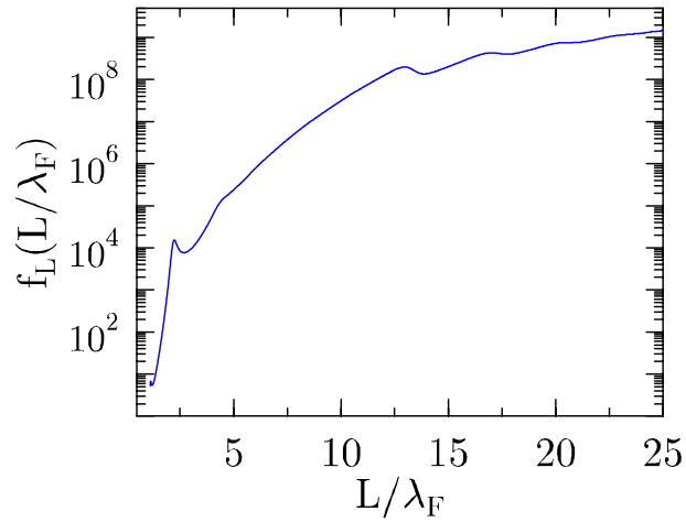
FIG. 10: Illustration of the effect of smearing of the interface. The same curve as in Figures 6 and 9, but for an even wider interface, d = 0.1 . Data as in Figure 3, but in logarithmic scale.
