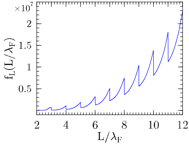
FIG. 1: Dimensionless conductivity of quantized films, Eq. (15), as a function of the film thickness L . The saw-like dependence is typical for the standard quantum size effect. The correlation radius of inhomogeneities R/\lambda_F = 1 , the thickness of the first layer L_1/\lambda_F = 2.1 , the width of the interface d = D/\lambda_F = 0.01 , and the strength of the barrier u_0 = 0.1 .
