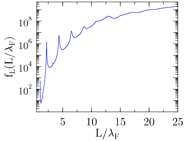
FIG. 9: Illustration of the effect of smearing of the interface. The same curve as in Figure 6, but for a wider interface, d = 0.01 .
