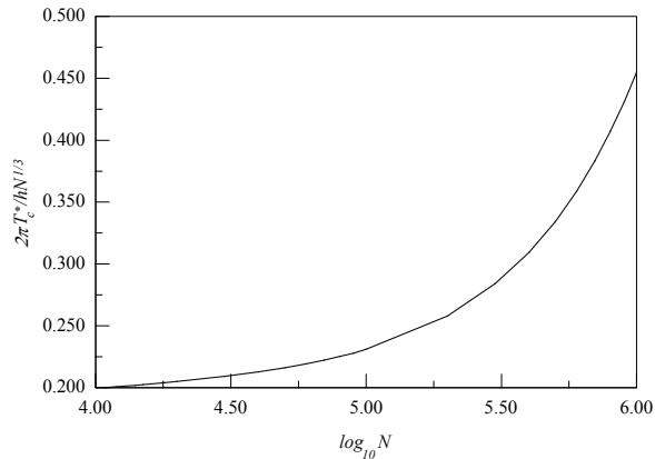
FIG. 5: Density dependence of the reduced critical temperature T_c^*/\hbar\omega N^{1/3} , Eq.(3), in the presence of the optical lattice. The behavior of T_c^* is drastically different from a similar trap without the optical lattice (Figure 2).
