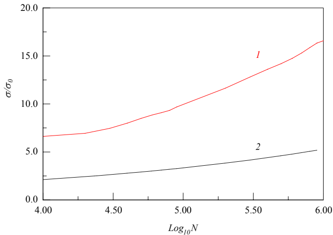
FIG. 3: Size of the condensate droplet \sigma(T=0) relative to the size of the trap \sigma_0 , \sigma/\sigma_0 , with (curve 1) and without (curve 2) the optical lattice as a function of the number of particles in the trap. The scattering lengths and effective masses are identical in both cases. Parameters of the lattice and the trap are given in the text.
